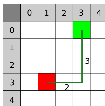
Figure 330: Example of Manhattan distance
